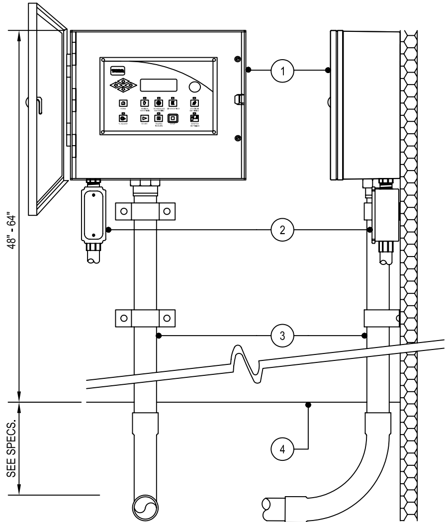
FRONT SECTION/ELEVATION NOT TO SCALE
