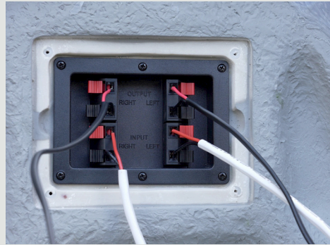
PROTECTED WIRING
