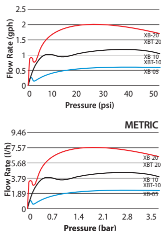
Xeri-Bug Emitter Performance
