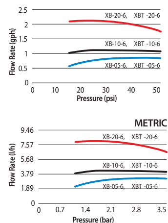
Multi-Outlet Xeri-Bug Emitter Performance
