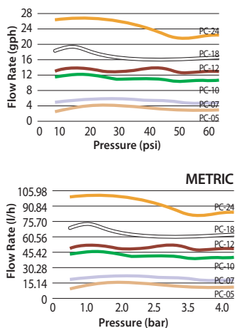
Pressure-Compensating Modules Performance
