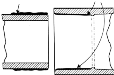
CEMENT COATINGS OF SUFFICIENT THICKNESS
