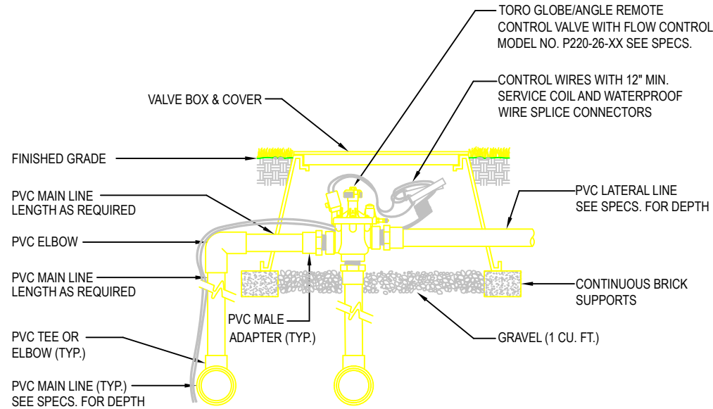
SECTION/ELEVATION NOT TO SCALE
