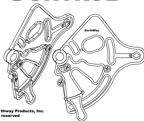
CLOSED ASSEMBLY - BOTTOM VIEW
