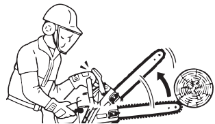
ROTATIONAL KICKBACK
