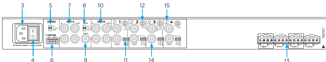
Sonance 8-50 Amplifier
