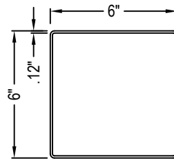
6" SQ. TUBE TOP VIEW
