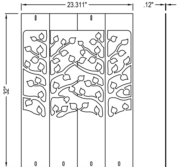
FLAT PATTERN FRONT VIEW
