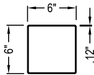
6" SQ. TUBE TOP VIEW
