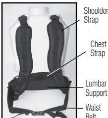
Figure 1 Strap Assembly
