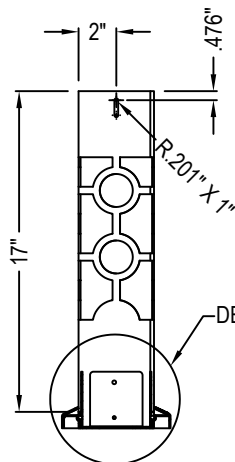
FRONT VIEW
