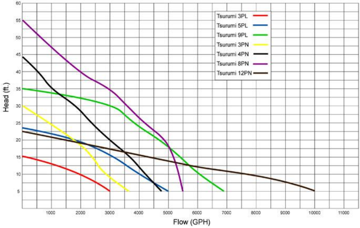
Tsurumi PL/PN Pump Flow Chart
