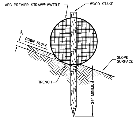
STAKE DETAIL (ON BARE SOIL) NO SCALE
