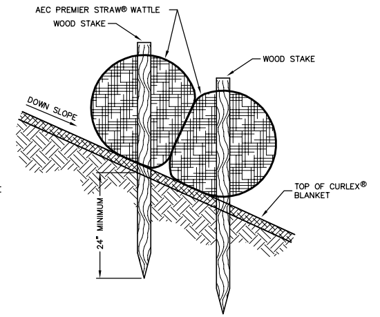
STAKE DETAIL (SECTION VIEW) NO SCALE
