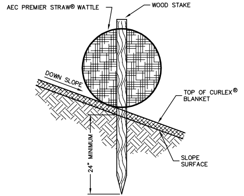
STAKE DETAIL (ON TOP OF CURLEX® ECB) NO SCALE
