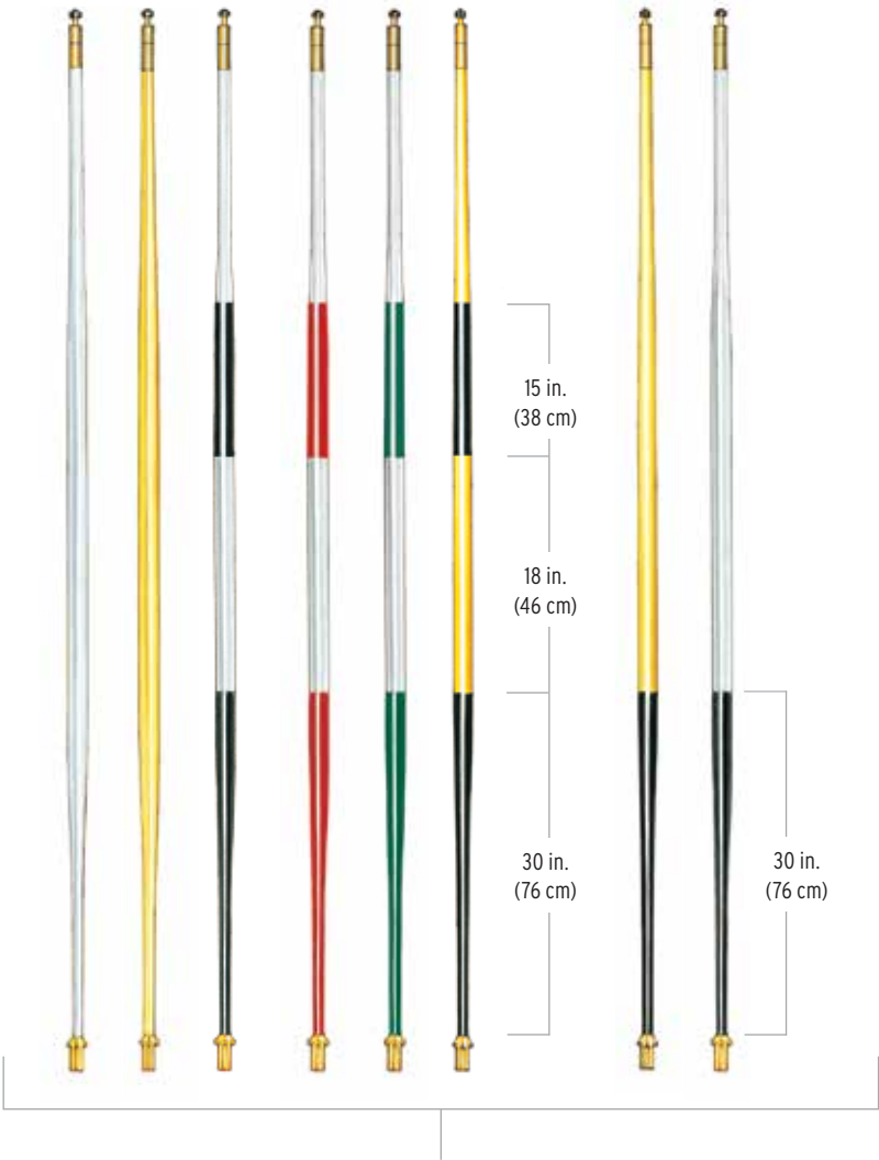
Tapered Fiberglass Tournament Flagsticks ¾ in. (2 cm)
