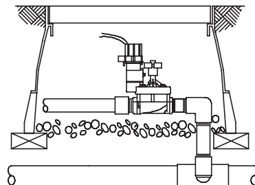
Plastic Electric Remote Control PEBIVM or PESBIVM Valve (with PRS-D)
